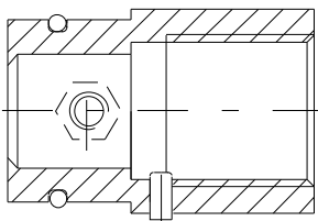
Coupling G1 / PMC 1,5"
