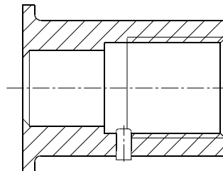
Coupling G1 / Hygienic coupling SMS standard:
