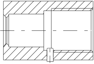
Standard coupling G1
